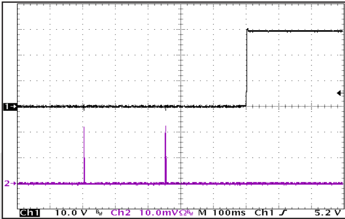
Figure 19: Rise of output voltage after the removal of a short circuit across the output terminals. R_{short} = 5\text{ m}\Omega . Ch 1: V_{out} (10 V/div). Ch 2: I_{out} (20 A/div). Bandwidth: 20 MHz.
