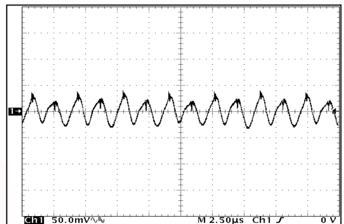
Figure 18: Output voltage ripple, V_{out} , at nominal input voltage and full load (50 mV/div). Bandwidth: 20 MHz. Load capacitance: 1 \mu F ceramic and 10 \mu F 100 m \Omega ESR tantalum. See Figure 16.
