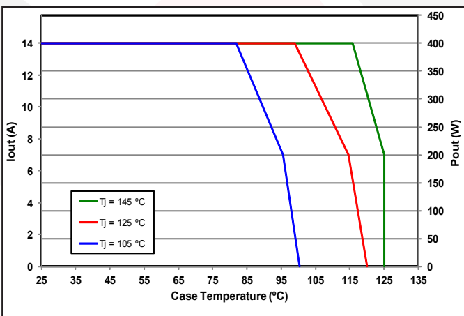
Figure 5: Output current and power derating curves vs. case temperature at nominal input voltage and at T_j=105\text{ }^{\circ}\text{C} , 125\text{ }^{\circ}\text{C} , and 145\text{ }^{\circ}\text{C} (see Note 9).
